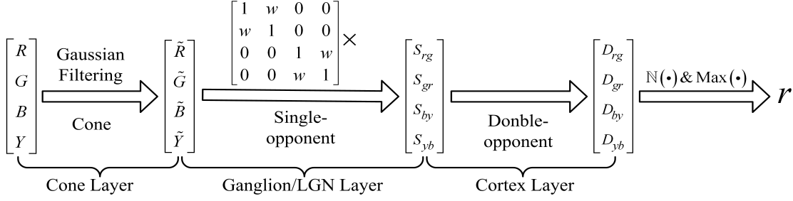
Figure 5. The full computational steps of the proposed system for color boundary detection. N(\cdot) denotes the linear normalization.
